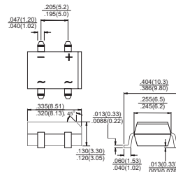
Dimensions in inches and (millimeters)
